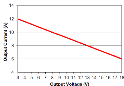
Figure 2. Graph showing maximum output current capability at different
