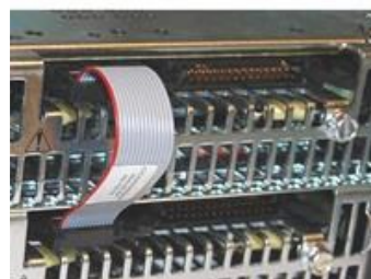
Shelf-to-shelf cable connection (part # CC848848952)
