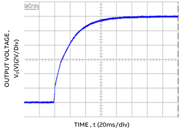
Figure 4. 12V start-up ( V_{in} : -48V_{dc} , full load)
