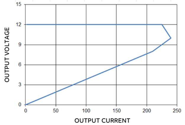
Figure 2. 12V output : Current limit profile ( V_{in} : -48V_{dc} )
